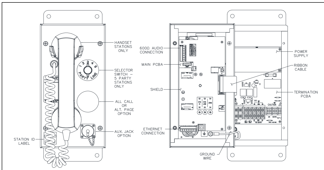
Figure 1. SP2 Class I Div. 2 Handset/Speaker Amplifier Station
